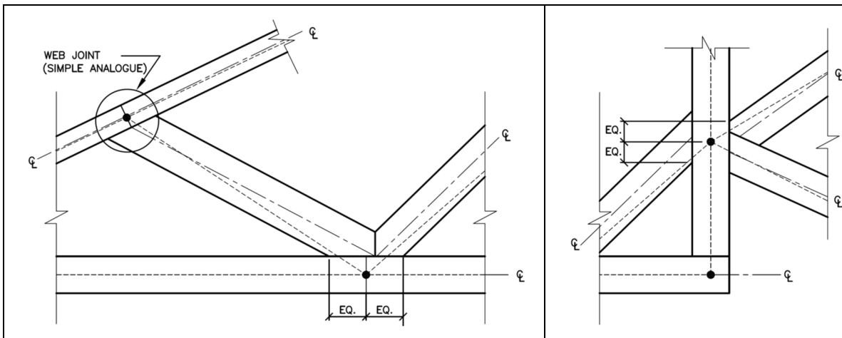
Figure A.2.5 – Web joints
