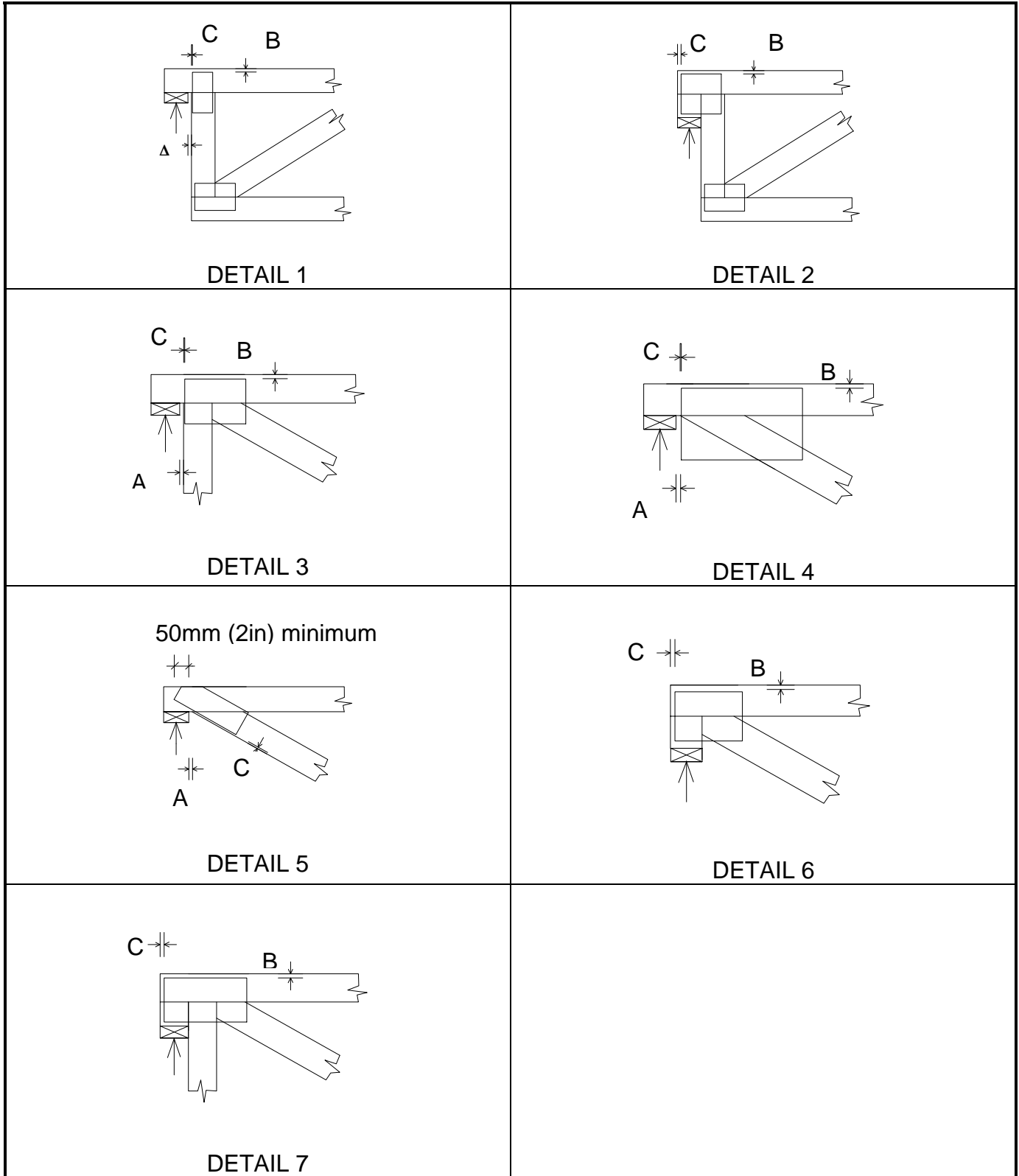
FIGURE D.1 TYPICAL TOP CHORD BEARING JOINT GUIDELINES FOR LUMBER ON EDGE
