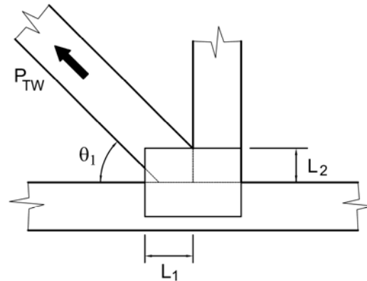
Figure 5.5.4 Shear-Tension Lengths and Angles
