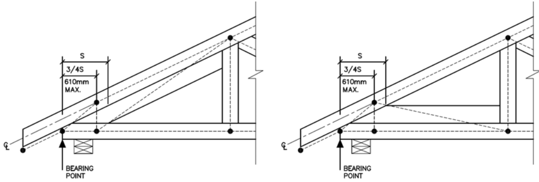
FIG. 4.1.2.1.E SHORT CANTILEVERED HEEL WITH TOP AND BOTTOM REINFORCING WEB. BEARING POINT AT FIRST ANALOGUE POINT.
