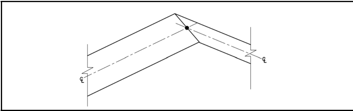
Figure 4.1.2.2.A Mitre Cut Pitch Break Joint
