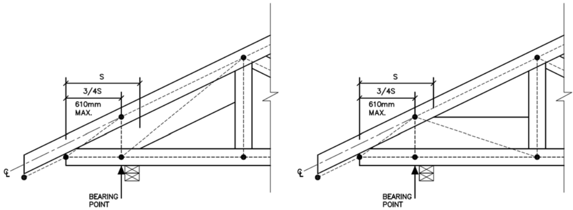
FIG. 4.1.2.1.F CANTILEVERED HEEL WITH TOP AND BOTTOM REINFORCING WEB. BEARING POINT AT SECOND ANALOGUE POINT.
