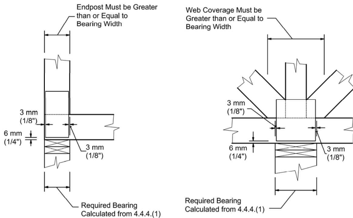
FIGURE 5.5.9 Bearing Reinforcement With Connector Plates
