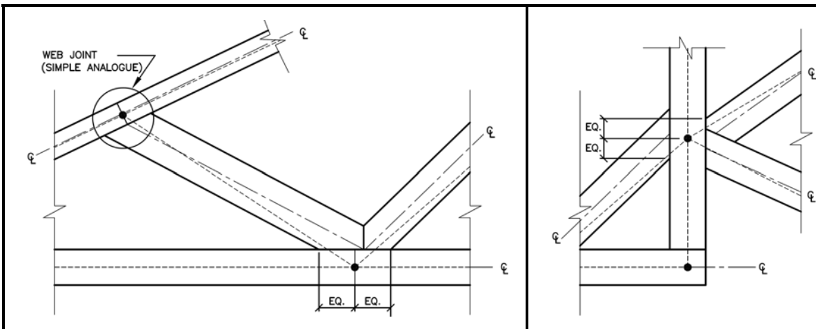
Figure 4.1.2.5 Web Joints
