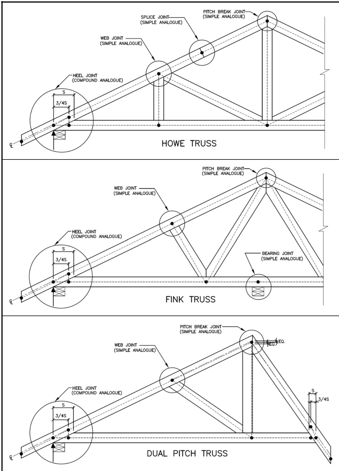
Figure 4.1.2 Simple and Compound Analogue
