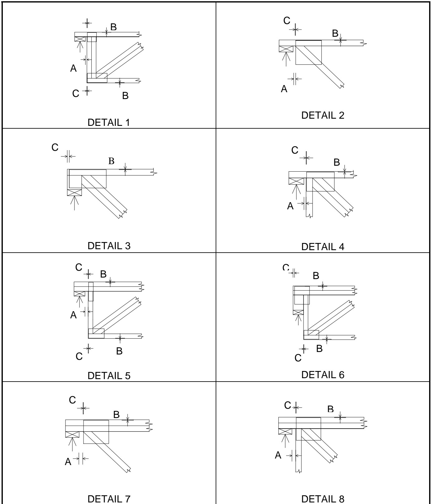
FIGURE D.2 TYPICAL TOP CHORD BEARING JOINT GUIDELINES FOR LUMBER ON FLAT
