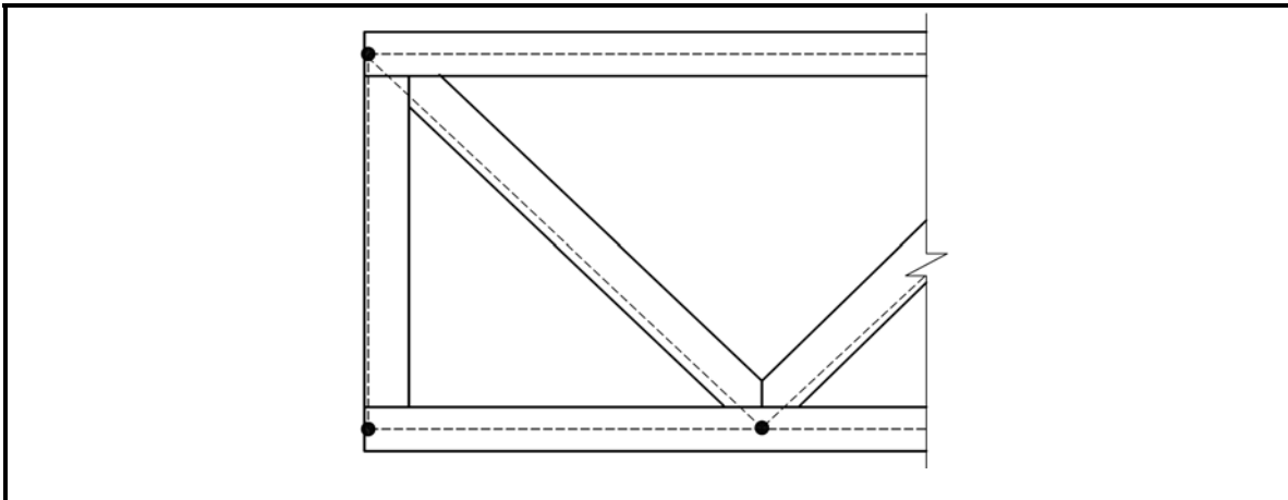
Figure 4.1.2.2.B Corner Joint
