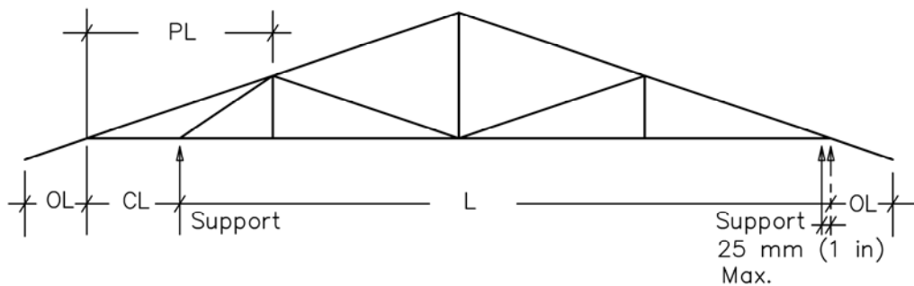
Figure 4.5.1.(4) Truss Deflection Lengths
