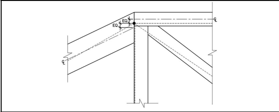
Figure 4.1.2.2 Pitch Break Joint
