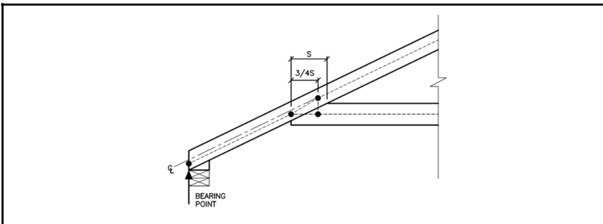
Figure 4.1.2.7 Tail Bearing Joint
