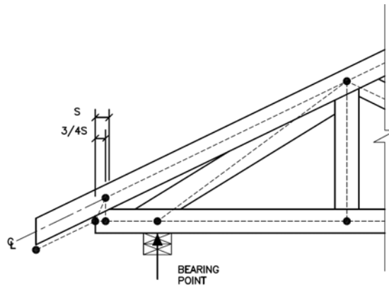
FIG. 4.1.2.1.G CANTILEVERED HEEL WITH TWO SEPARATE JOINTS.
