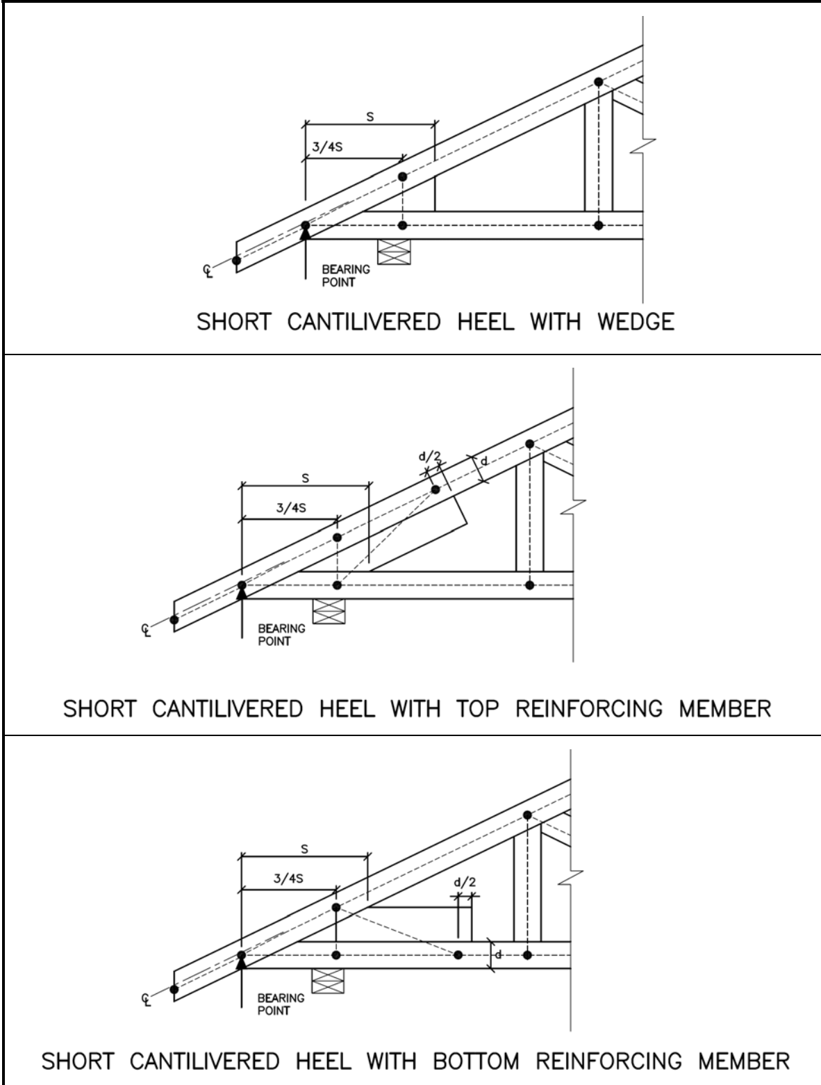
Figure 4.1.2.1.D Short Cantilevered Heels
