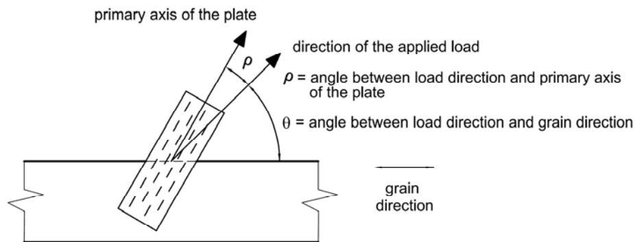
Figure 5.1.(5) Truss Plate, Load and Grain Orientation
