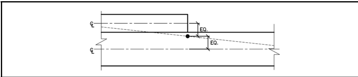
Figure 4.1.2.4 Lapped Joint
