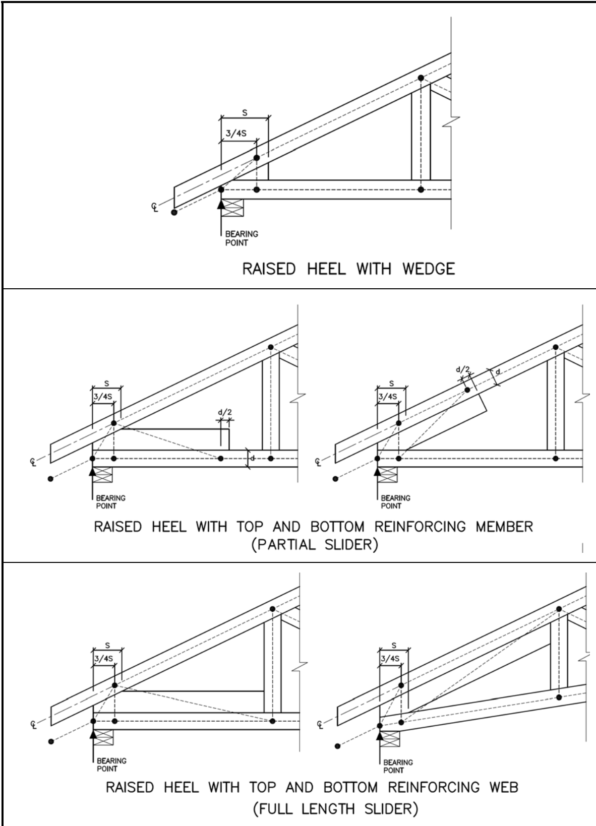
Figure 4.1.2.1.C Raised Heels
